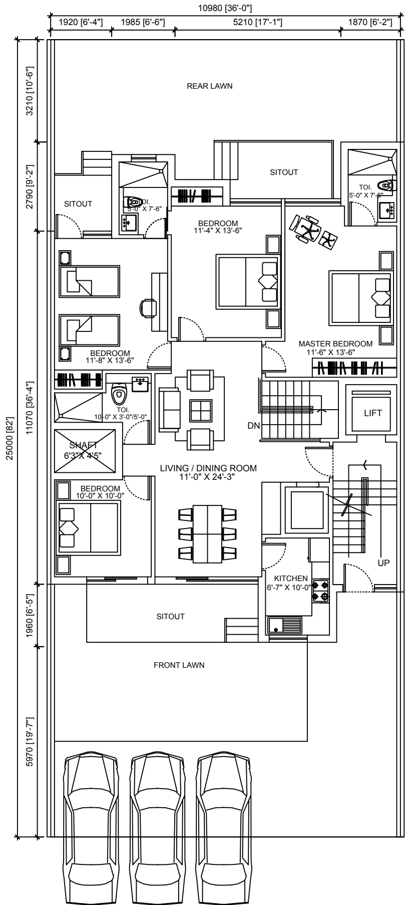
GROUND FLOOR
